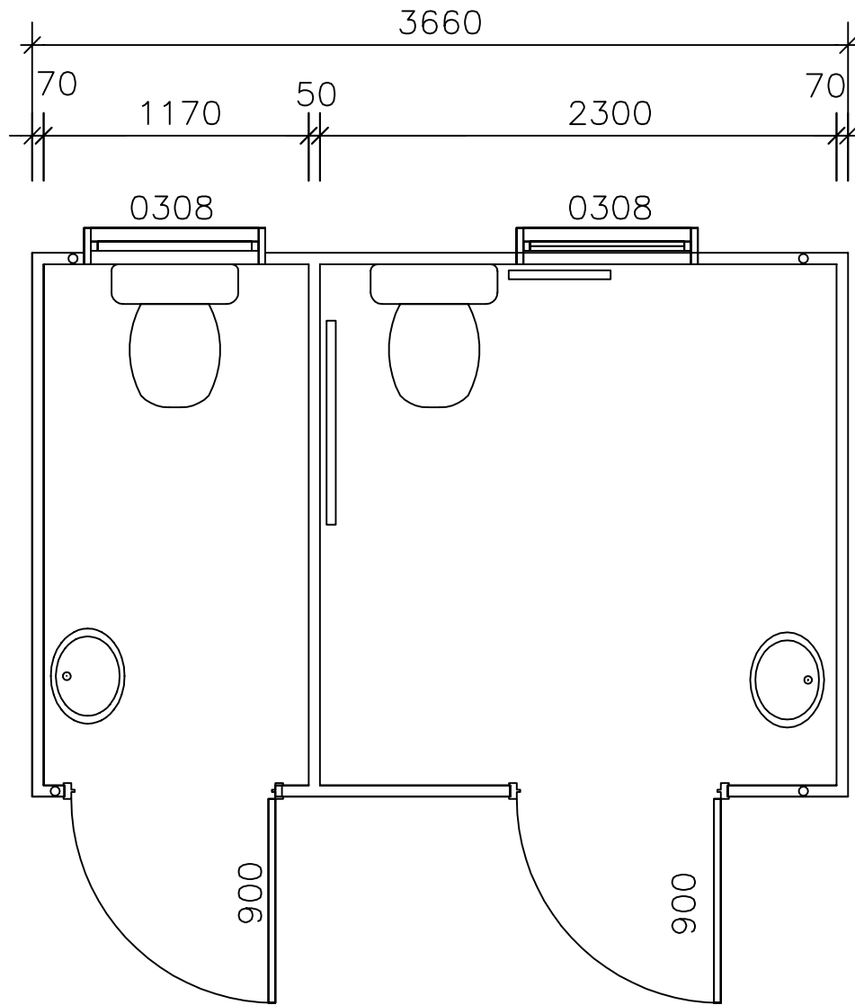
DISABLED/UNISEX DOUBLE TOILET UNIT
