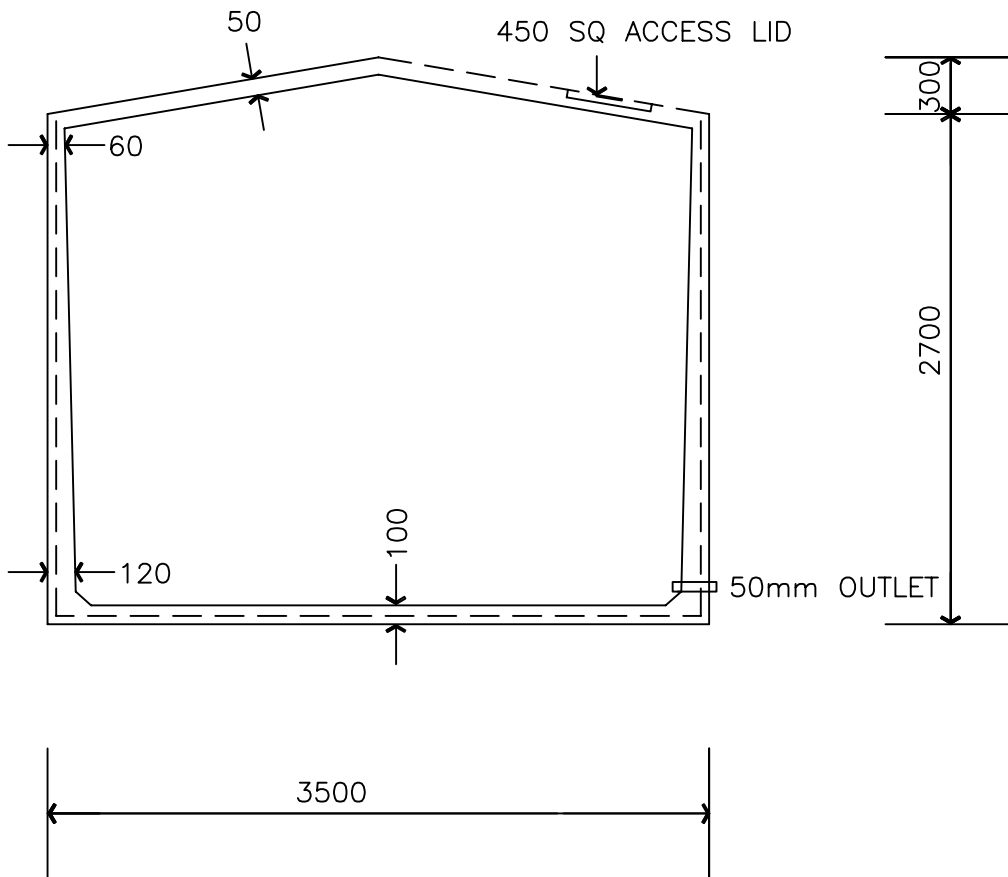
22,500 LITRE CONCRETE TANK SCALE 1:50
