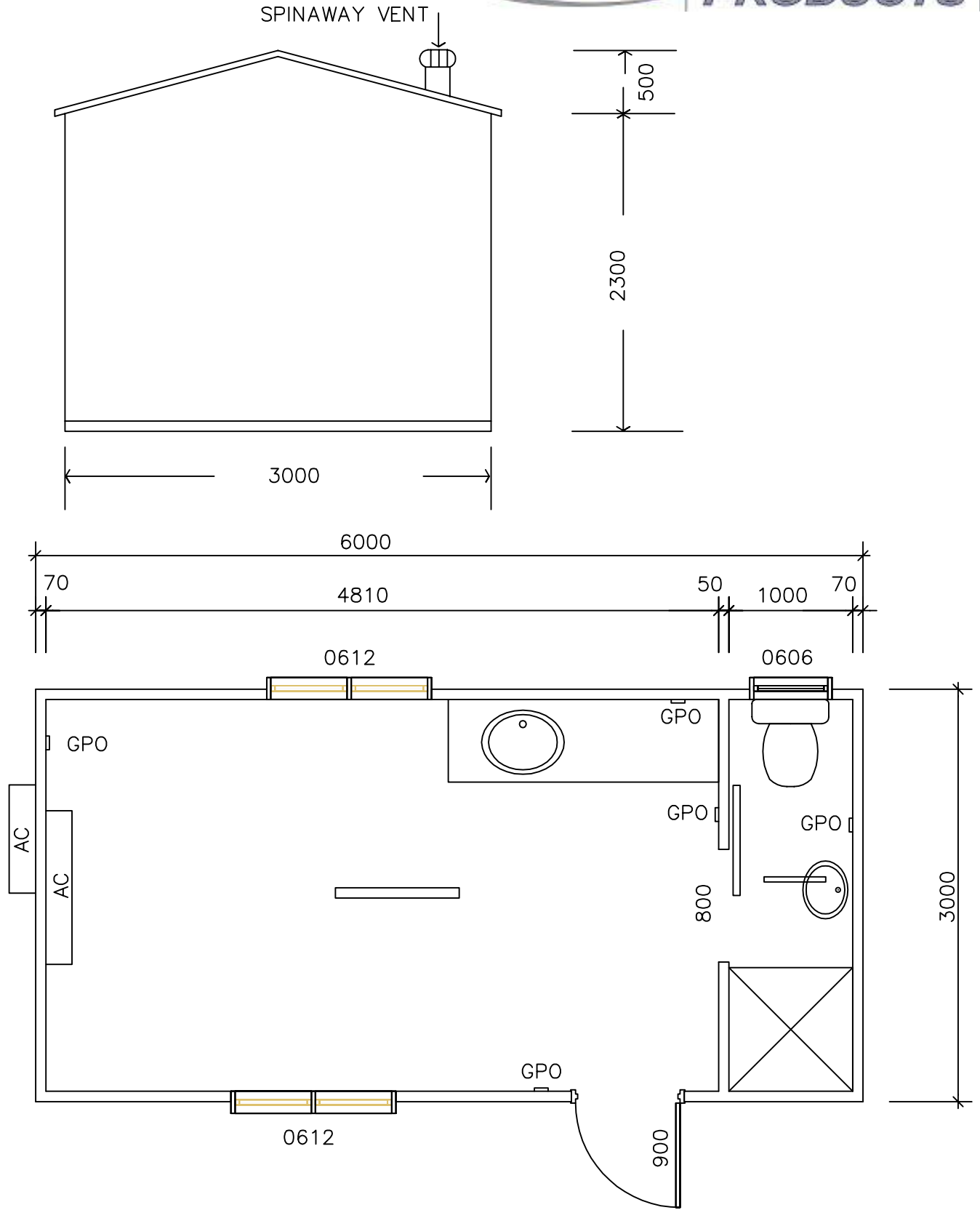
FLOOR PLAN Scale 1:40
